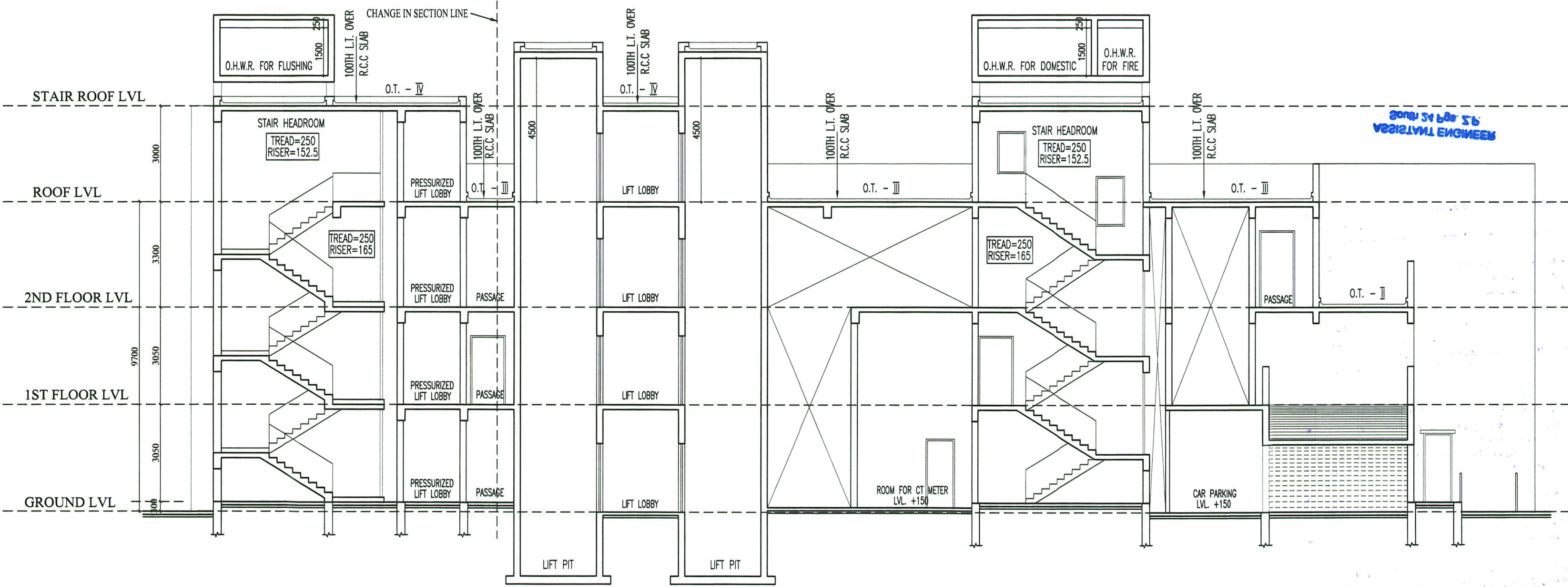
SECTION AT S1-S1 TOWER - 1
