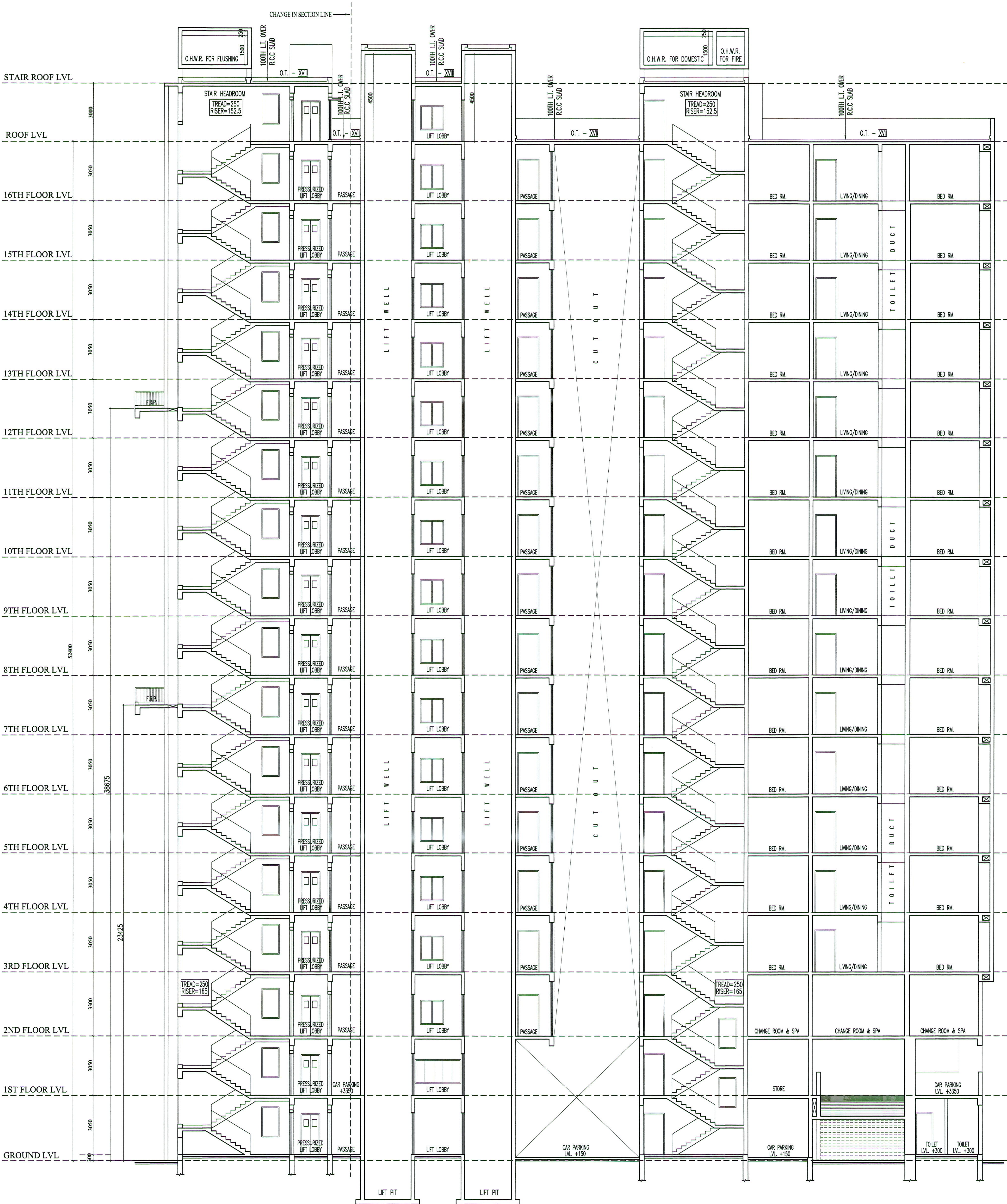
SECTION AT S3-S3 TOWER - 2
